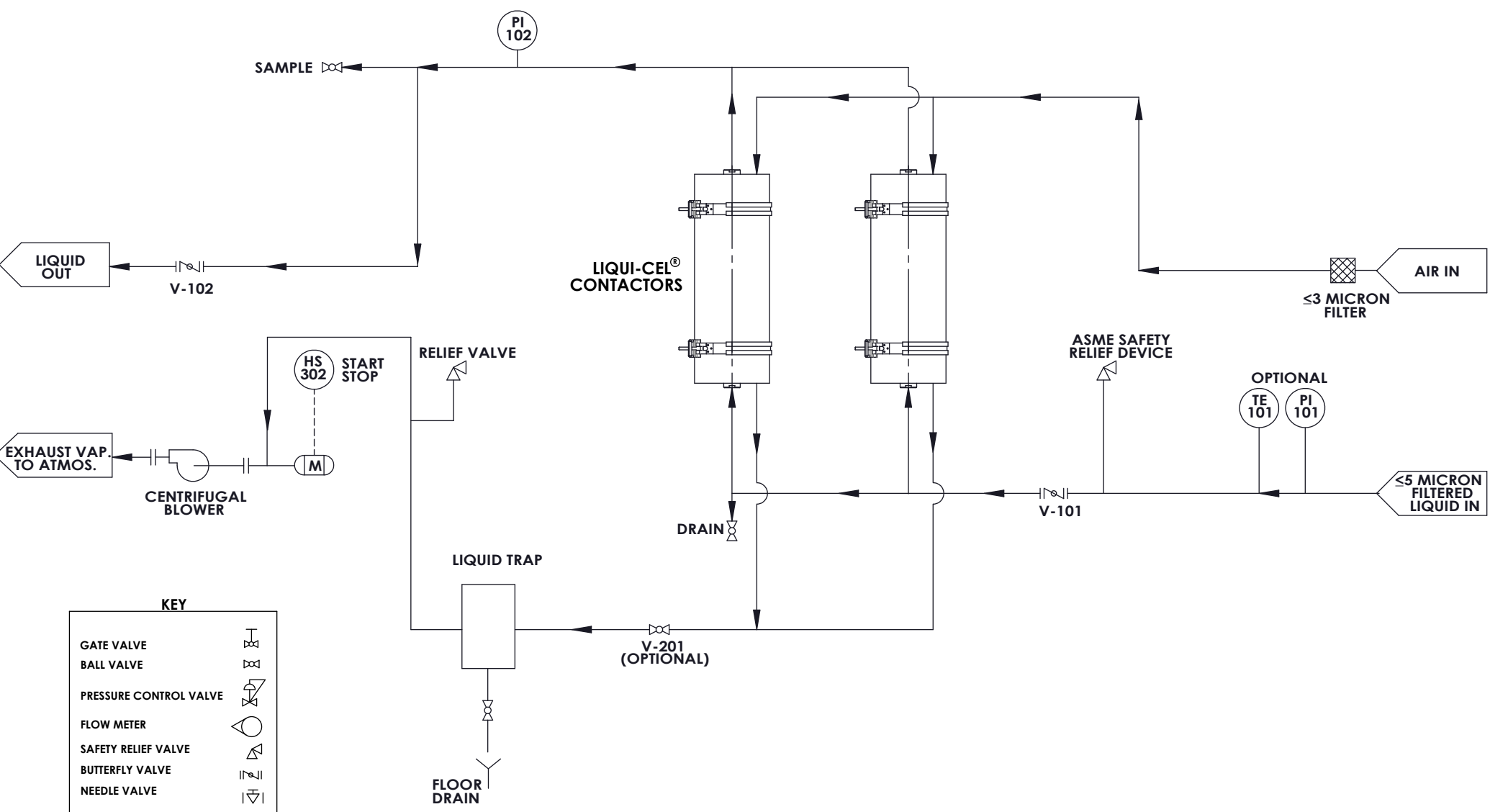
AIR BLOWER COMBO MODE USING BLOWER TO PULL IN ATMOSPHERIC AIR (PARALLEL CONFIGURATION)
